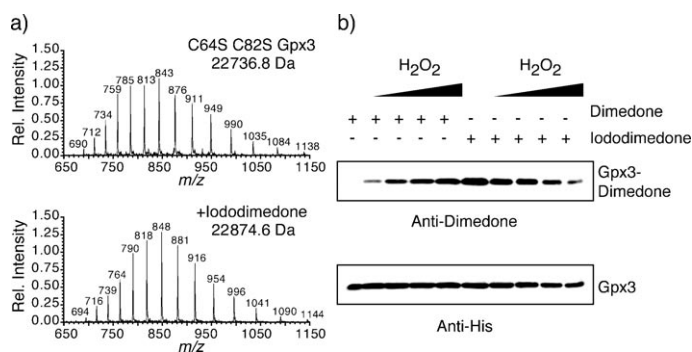
Figure 1. ESI-LC/MS and Western blot analysis shows that iododimmedone selectively labels the thiol group of C36 in C64S C82S Gpx3. a) The molecular weight of mock-treated C64S C82S Gpx3 is 22736.8 Da corresponding to intact, unmodified protein (top spectrum). The molecular weight of C64S C82S Gpx3 incubated with iododimmedone is 22874.6 Da (bottom spectrum), corresponding to C64S C82S Gpx3 with a single dimedone adduct ( \Delta m = 138 Da). b) C64S C82S Gpx3 (50 \mu M) untreated or oxidized with H 2 O 2 (12.5, 25, 50, or 100 \mu M) followed by dimedone (20 mM) or iododimmedone (20 mM). The resulting samples were analyzed by Western blot using an antibody that recognizes the protein–dimedone adduct (top panel). Total protein content was determined by an anti-His antibody (bottom panel).
