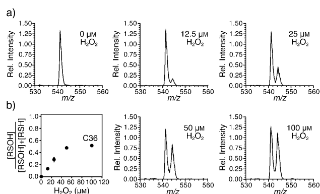
Figure 2. Quantifying sulfenic acid modification of C64S C82S Gpx3. a) C64S C82S Gpx3 (50 \mu\text{M} ) was untreated or oxidized with \text{H}_2\text{O}_2 and incubated with [\text{D}_6] dimedone (20 mM). Small molecules were removed and the resulting protein treated with iododimmedone (50 mM). Labeled protein was digested with trypsin and tagged peptides were identified and quantified by LC-MS. The molecular ions corresponding to m/z of 541 and 544 are consistent with the mass of peptide 36–43 modified by iododimmedone (representing the thiol form) or [\text{D}_6] dimedone (representing the sulfenic acid form), respectively. b) Fraction of sulfenic acid detected at C36 (●) plotted as a function of \text{H}_2\text{O}_2 concentration. The extent of sulfenic acid formation was determined by dividing the heavy-isotope labeled peak by the sum of the heavy- and light-isotope labeled peak intensities in the mass spectrum (i.e., [\text{RSOH}]/([\text{RSH}] + [\text{RSOH}]) ). Error bars represent \pm s.d. calculated from duplicate experiments.
